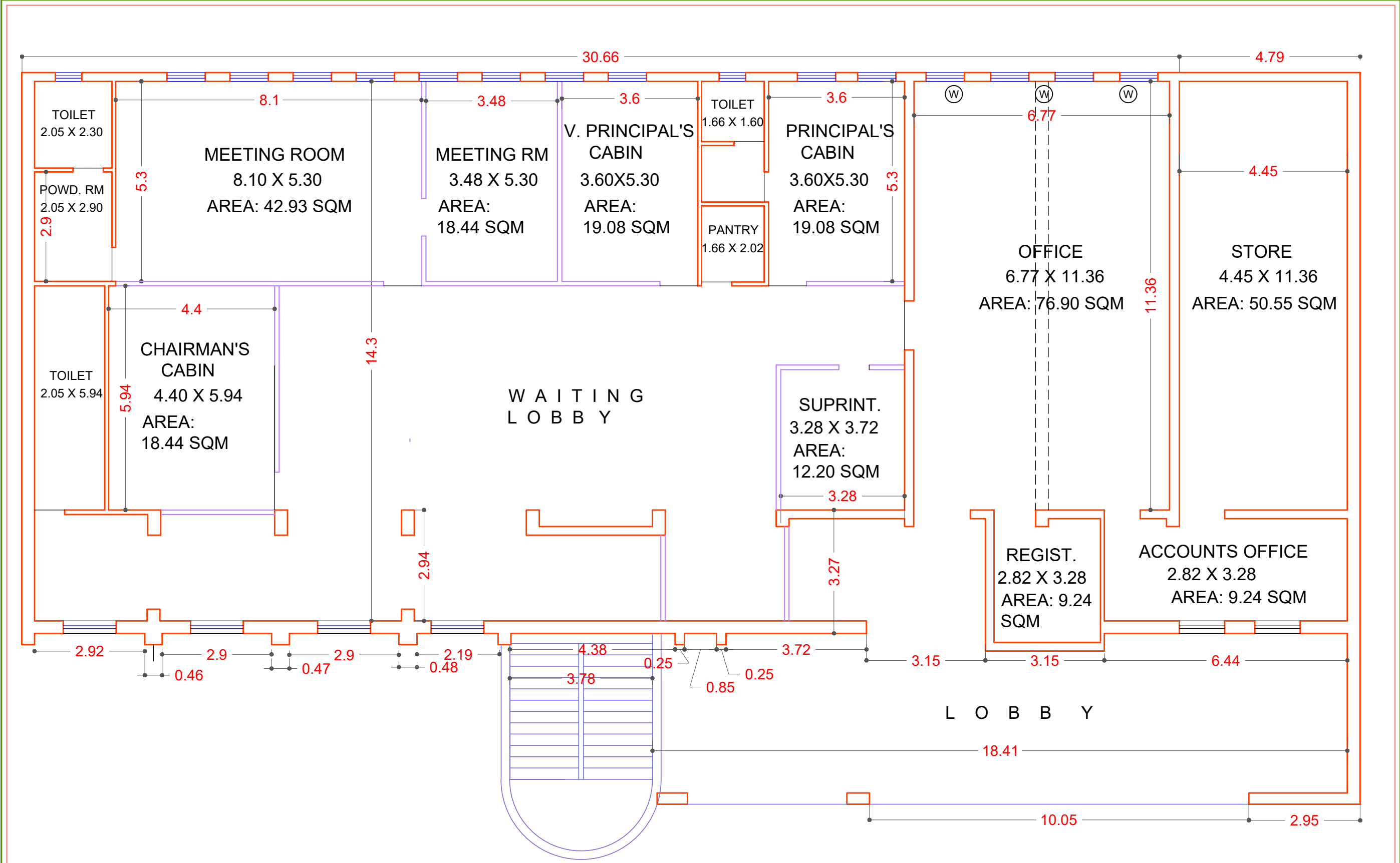
GROUND FLOOR ( MAIN BUILDING)
